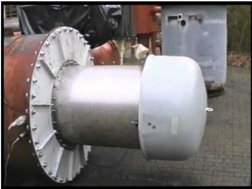
Explosion trials of a silo vent filter INFA-JETRON Typ AJB to prove pressure shock resistance.
